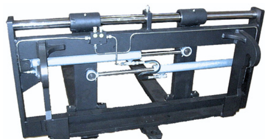
Merlo ZM 2
